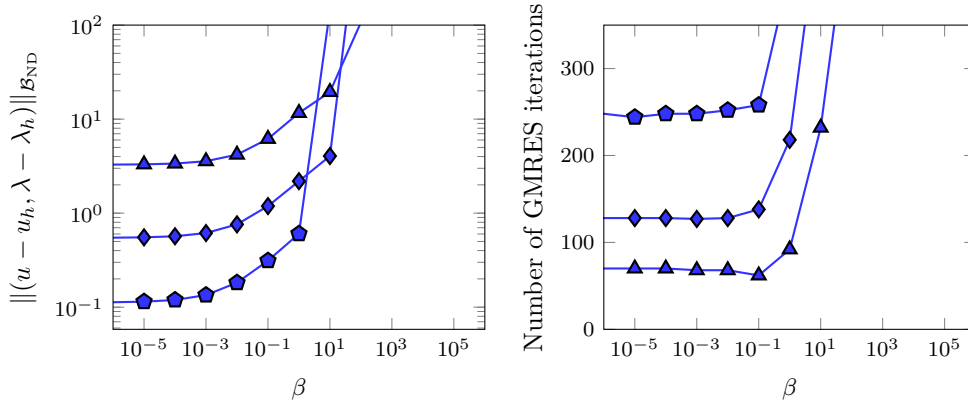
FIG. 3. The dependence of the error (left) and iteration count (right) on the value of \beta for h = 2^{-2} (blue triangles), h = 2^{-3.5} (blue diamonds), and h = 2^{-5} (blue pentagons), for the mixed Dirichlet–Neumann problem on the unit sphere, with k = l + 1 = 1 . Here we use \beta_D = \beta h^{-1} and \beta_N = \beta h .
